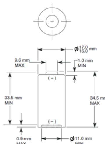
Dimensions shown are IEC standards
