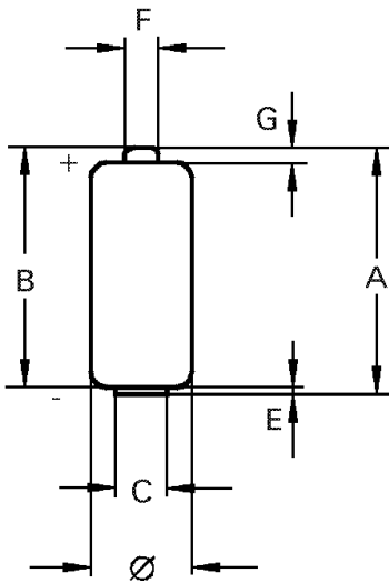
Dimensions [mm]
